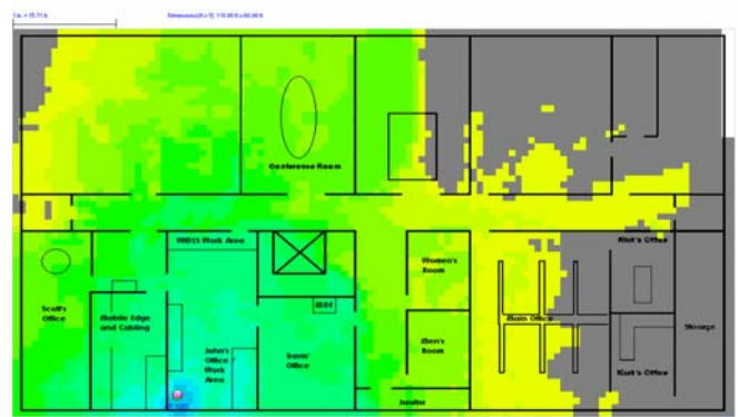
Site Survey Coverage: WAP inside Oberon model 1025-00 Fiberglass reinforced NEMA 4 enclosure
