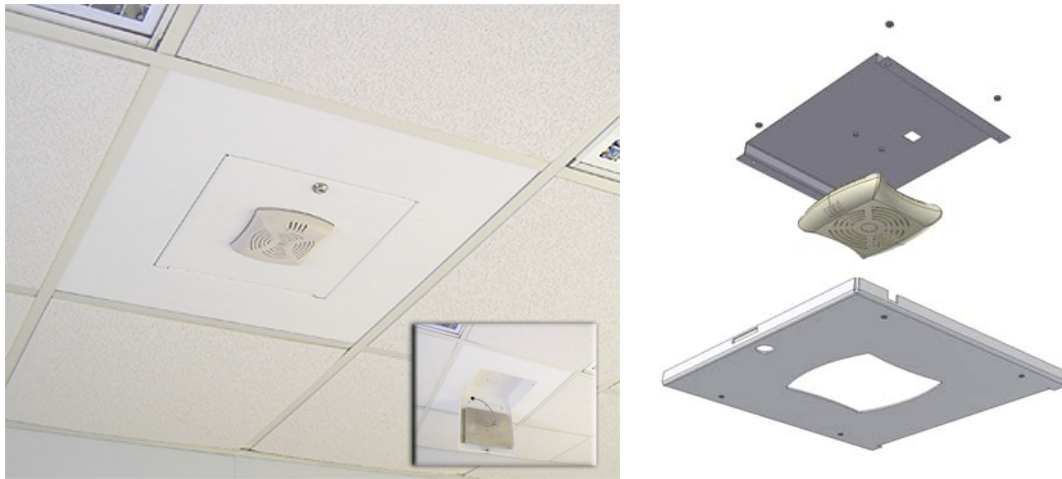
1) Model 1053-AP105 shown with Aruba Networks AP105 access point (not included) 2) Exploded view of the door, access point, and bracket
