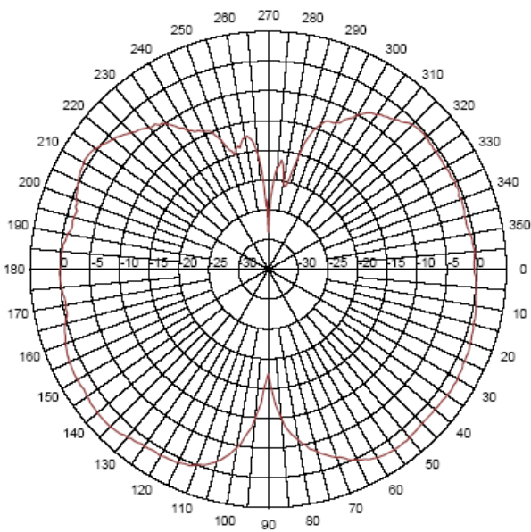
ELEVATION PATTERN
