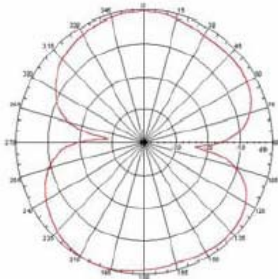
ELEVATION PATTERN (5.15 GHz)
