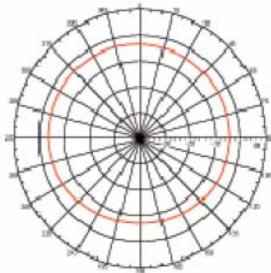
AZIMUTH PATTERN (2.45 GHz)
